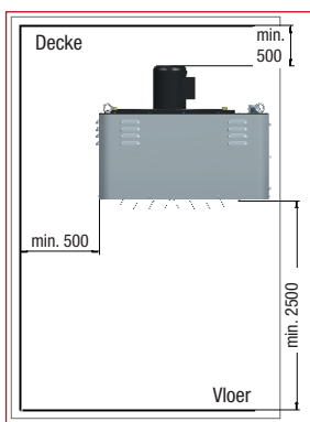
Detail ventilator
