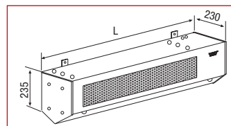
Dimensions (mm)
